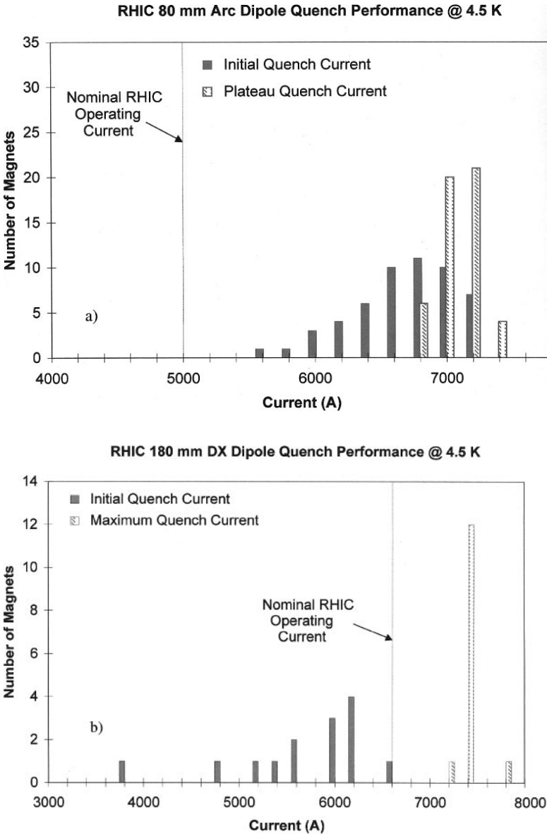
Figure 6 Quench performance for (a) arc dipoles and (b) beam-separation dipoles.
