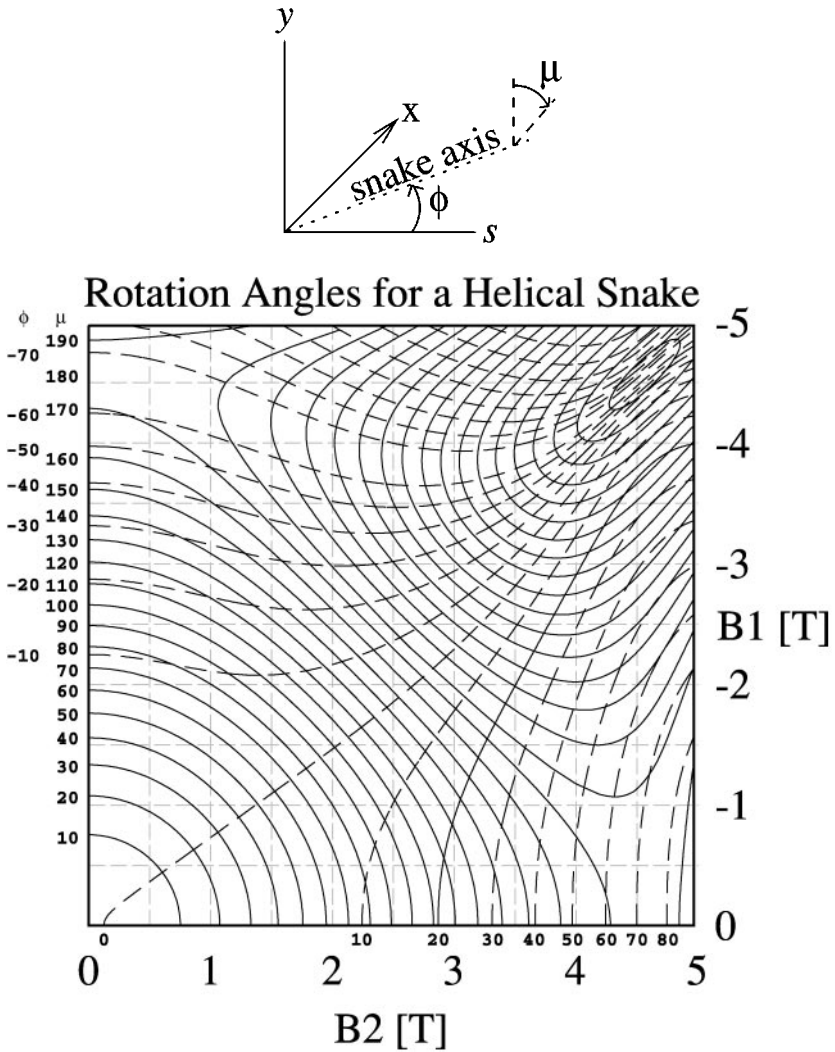
Figure 21 Change of the direction of the snake rotation axis as a function of magnet excitation. This calculation uses a simplified analytical expression for the snake magnetic field. The rotation axis of the snake is \phi and the rotation angle is \mu . B_1 is the field strength of the outer pair of helices, and B_2 is the field strength of the inner pair.
