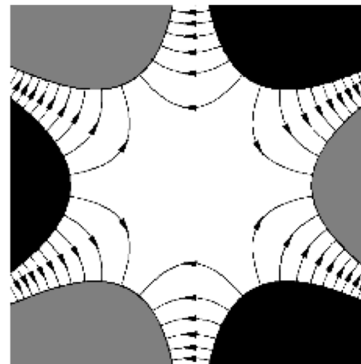
Sextupole and skew sextupole n = 3
