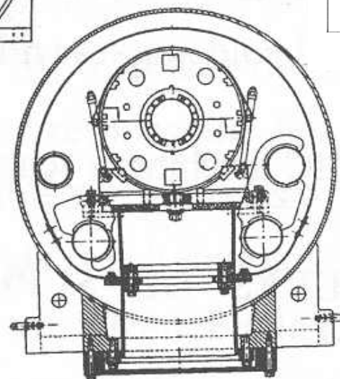
RHIC
