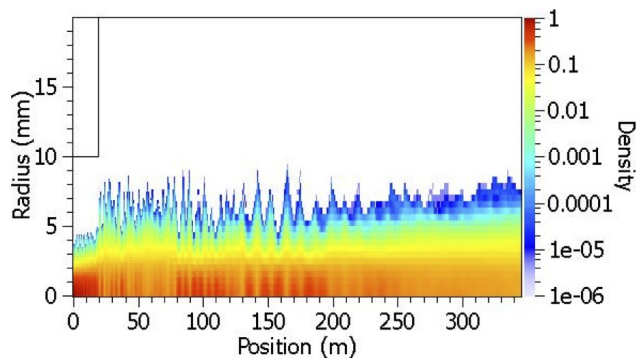
Figure 3: Simulated beam density and halo generation along an idealised linac.
