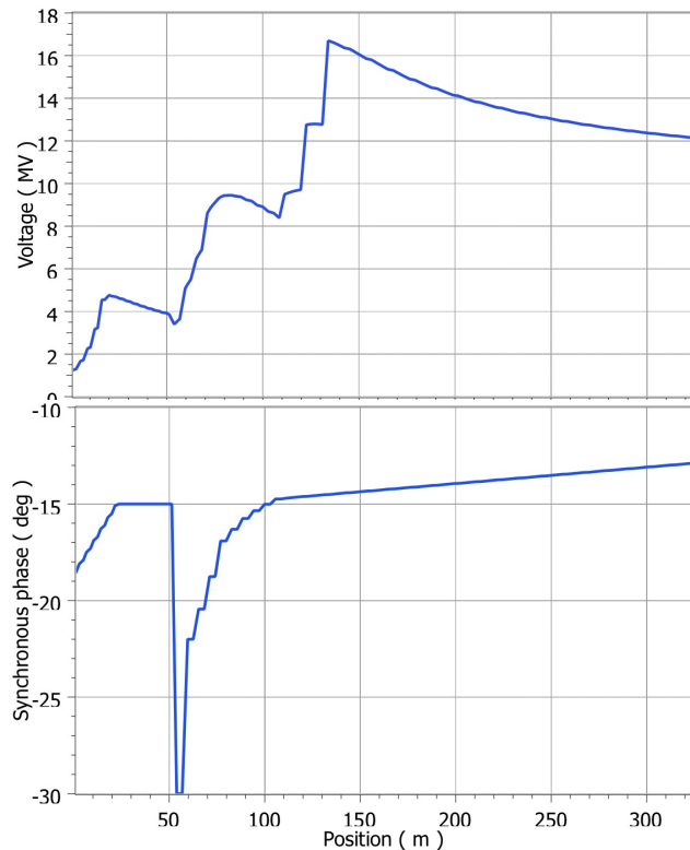
Figure 2: Spoke resonator and elliptical cavity voltage (TOP) and phase (BOTTOM) optics settings for the simulation of a 50 mA beam under ideal conditions. (Phase is everywhere reported with f = 352.21 MHz.)
