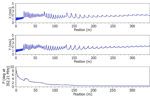
Figure 4: RMS beam sizes along the linac: horizontal (top), vertical (middle), and longitudinal (bottom). The RMS longitudinal phase spread is plotted at 352.21 MHz
