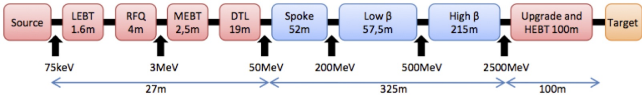
Figure 1: Provisional block layout of the ESS Linac (not to scale).
