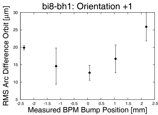
(a) With a database offset of -1.36 mm, bi8-bh1 BBA would have given a result near +2.8 mm if its offset had been reversed.
