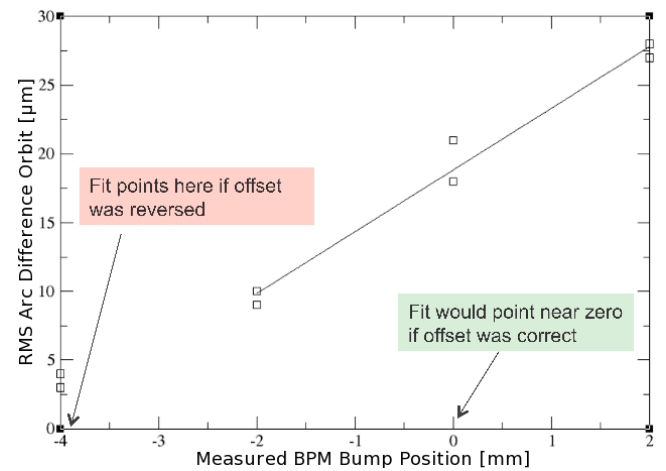
Figure 2: BBA plot for bo2-bv1 that was part of the confirmation of vertical BPM offset reversal. The controls system offset at the time of data taking was 1956 \mu\text{m} . The BBA result above is twice the magnitude and the opposite sign of this value which is strong evidence for offset reversal.
