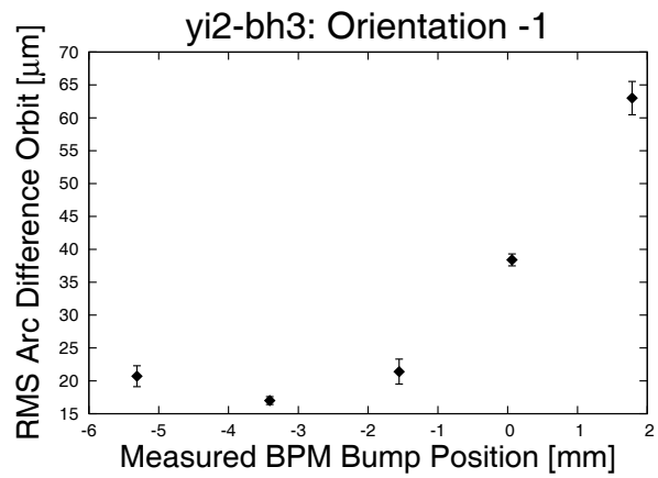
(b) A result of -3.5 mm, roughly twice the magnitude and opposite sign of the database offset of 1.79 mm, suggests offset reversal for yi2-bh3.
