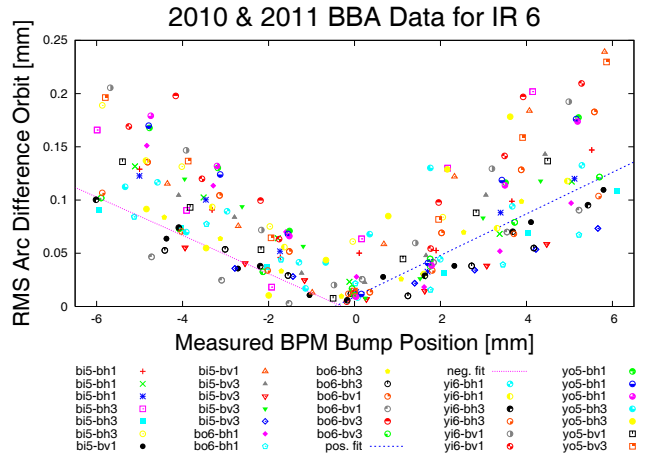
Figure 1: BBA data for all Q1 and Q3 BPMs at 6 o’clock in both Yellow and Blue. The resulting offsets for these BPMs are listed in table 1. Most BPMs are shown multiple times and only one fit (bo6-bv3 from March 09, 2010) is included. The RHIC BPM naming convention can be explained by way of an example: Yellow Inside 2 o’clock BPM Horizontal 3 is abbreviated yi2-bh3.
